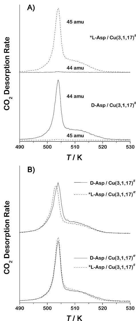
Figure 3. Temperature-programmed reaction spectroscopy (TPRS) of D- and *L-Asp on the Cu(3,1,17) R&S surfaces at saturation coverage. A) Monitoring of CO 2 ( m/q = 44 amu) and *CO 2 ( m/q = 45 amu) clearly differentiates enantiomers. B) Equivalent combinations of adsorbate and substrate show no isotope effect on the decomposition kinetics.
