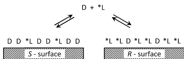
Figure 2. Adsorbed D- and *L-enantiomers on chiral surfaces at equilibrium with a racemic mixture in the gas phase. The higher adsorption energy of the D-enantiomer on the S-surface results in a higher coverage of the D-enantiomer than the *L-enantiomer (left). As a result of the diastereomeric relationship between the adsorption energies, the *L-enantiomer has a higher coverage than the D-enantiomer on the R-surface (right).
